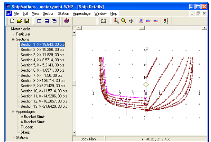
Figure 2 – Creating hull form
